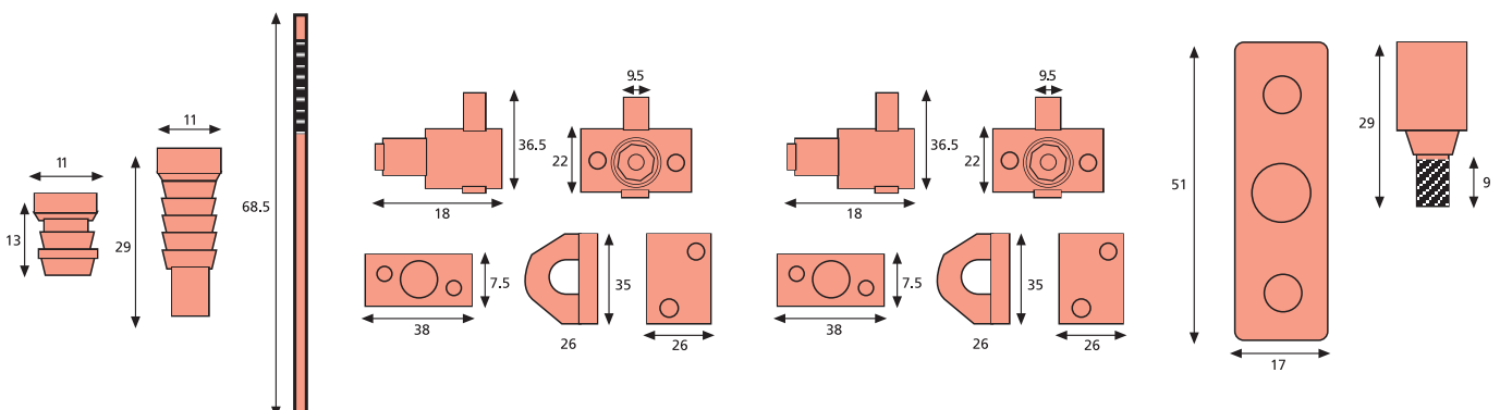
Dual Screw
