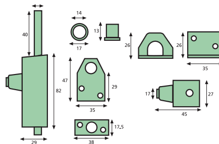
Multi-Purpose Bolt
